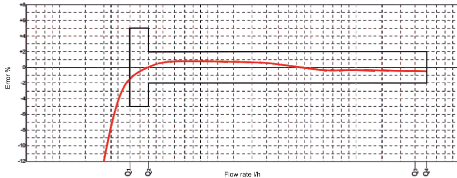
Error Curve
