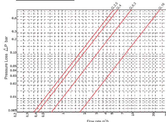
Pressure Loss
